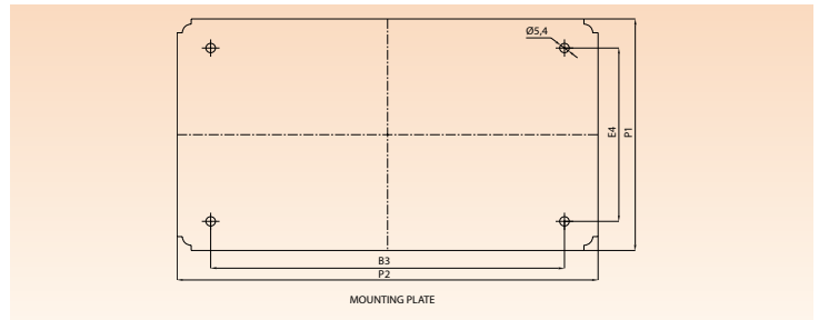
Mounting Plate
