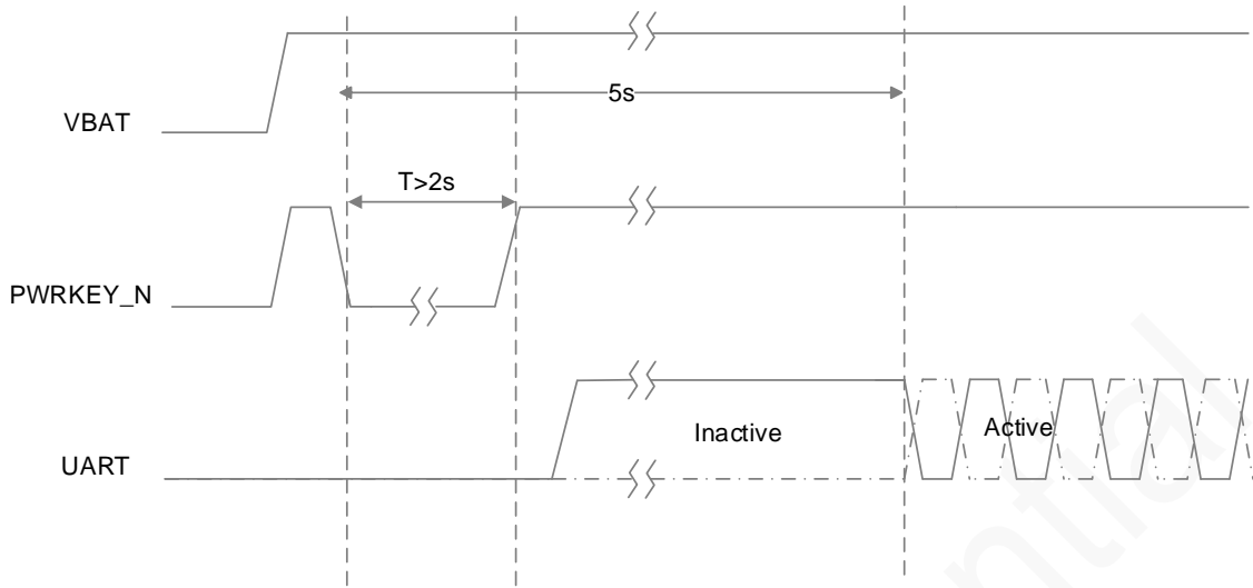
Figure 5-8 Power-on process
