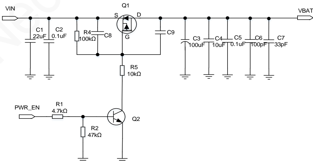
Figure 5-3 Recommended power supply design 2
