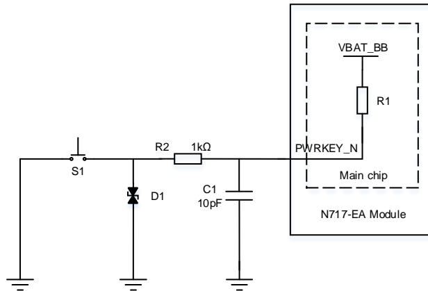
Figure 5-6 Reference design of key-control startup
