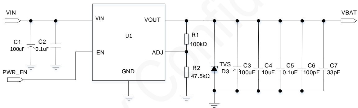
Figure 5-4 Recommended power supply design3
