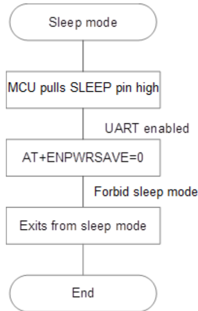
Figure 5-36 Process of waking up the module
