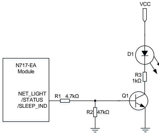
Figure 5-37 Driving LED indicators with a triode
