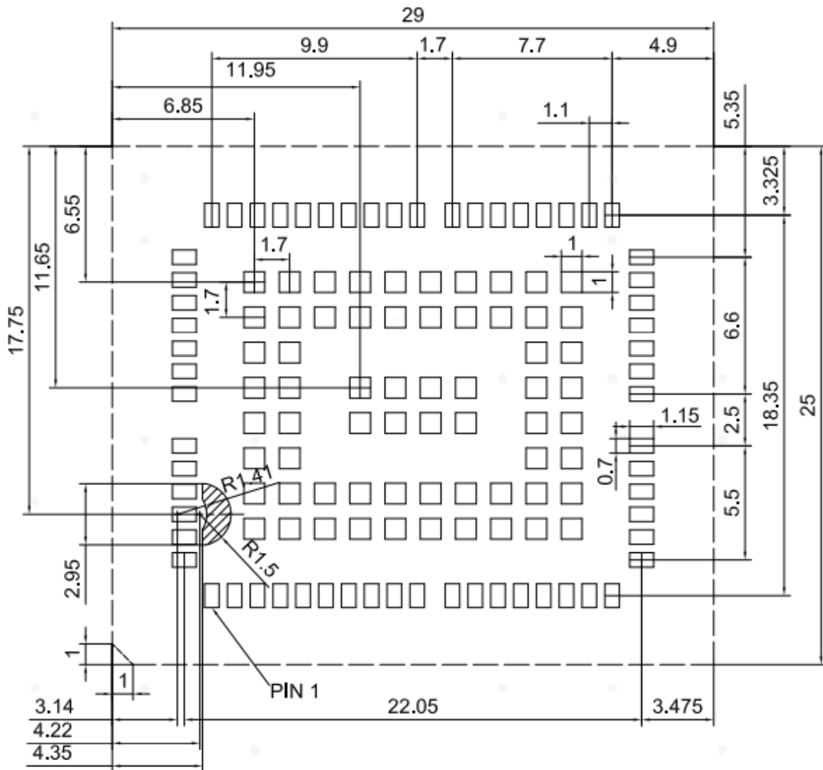
Figure 9-2 Application PCB package (top view, unit: mm)
