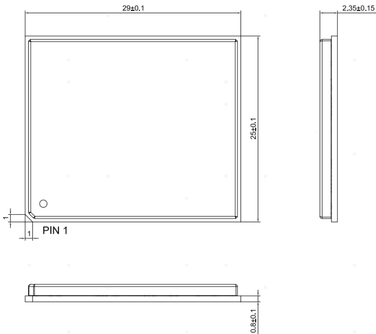
Figure 8-1 N717-EA top and side view dimensions (unit: mm)
