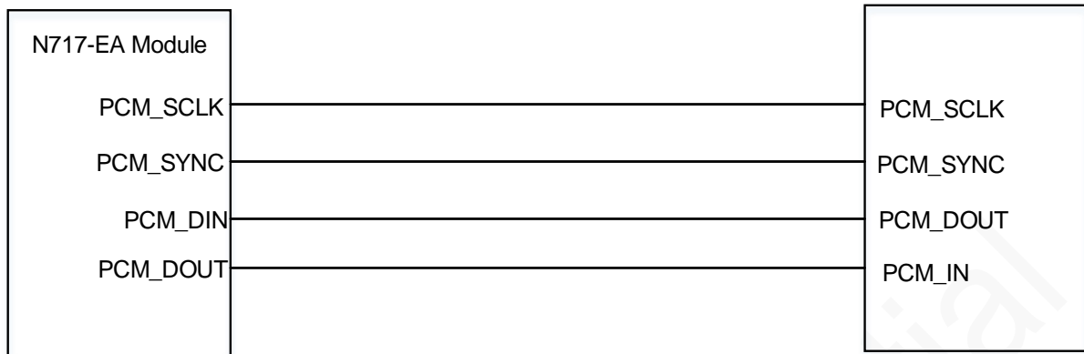
Figure 5-22 Reference design of the PCM interface
