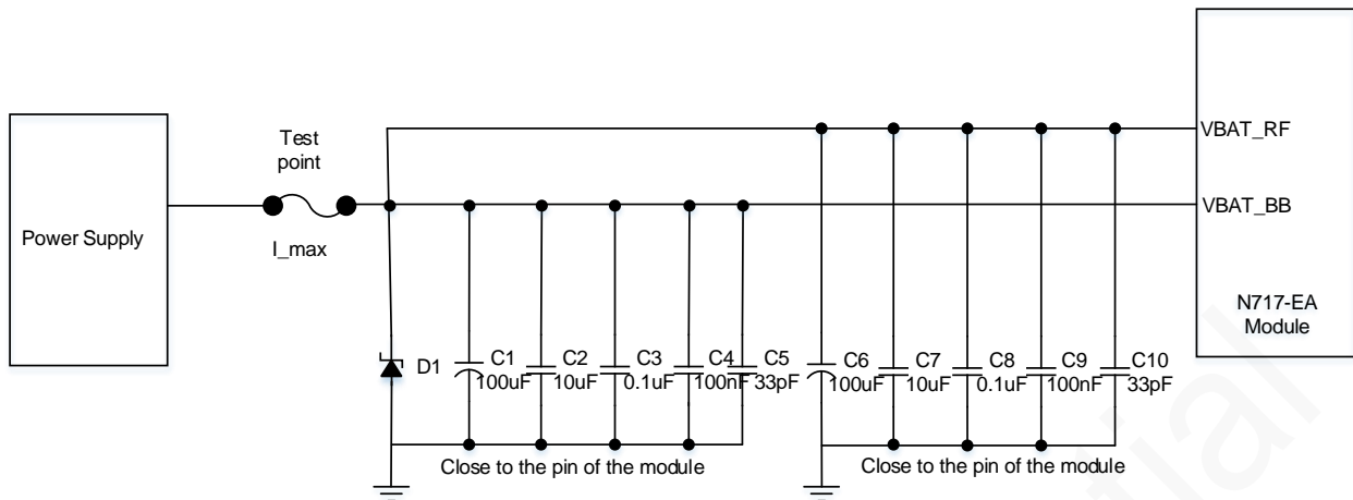
Figure 5-2 Recommended power supply design 1
