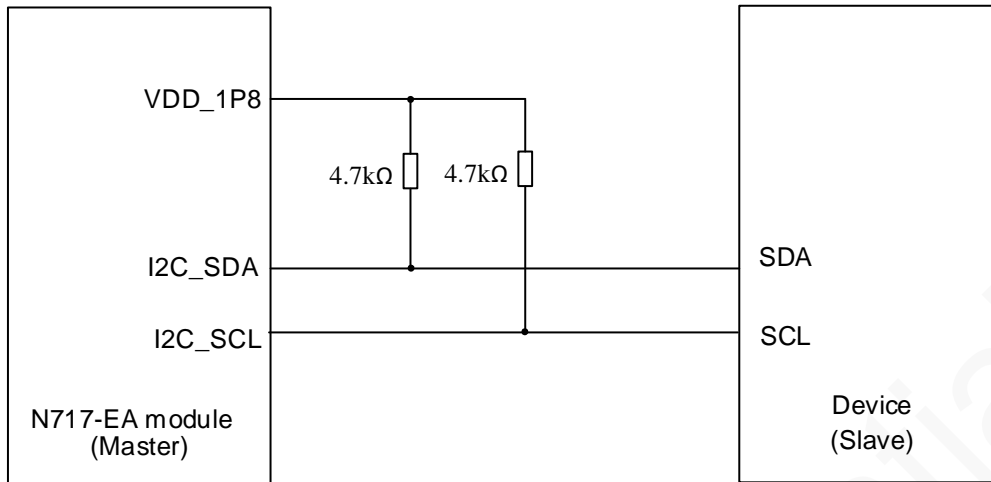
Figure 5-23 Reference design of the I2C interface
