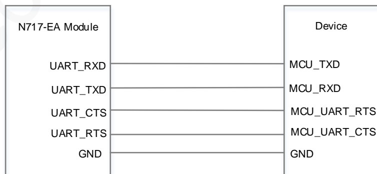
Figure 5-15 Reference design of the UART interface
