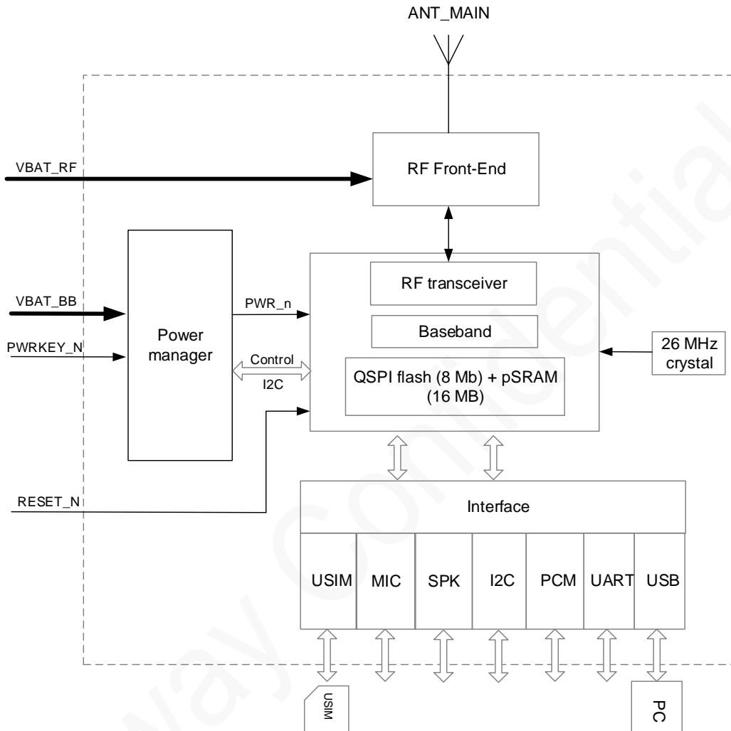
Figure 2-1 Block diagram
