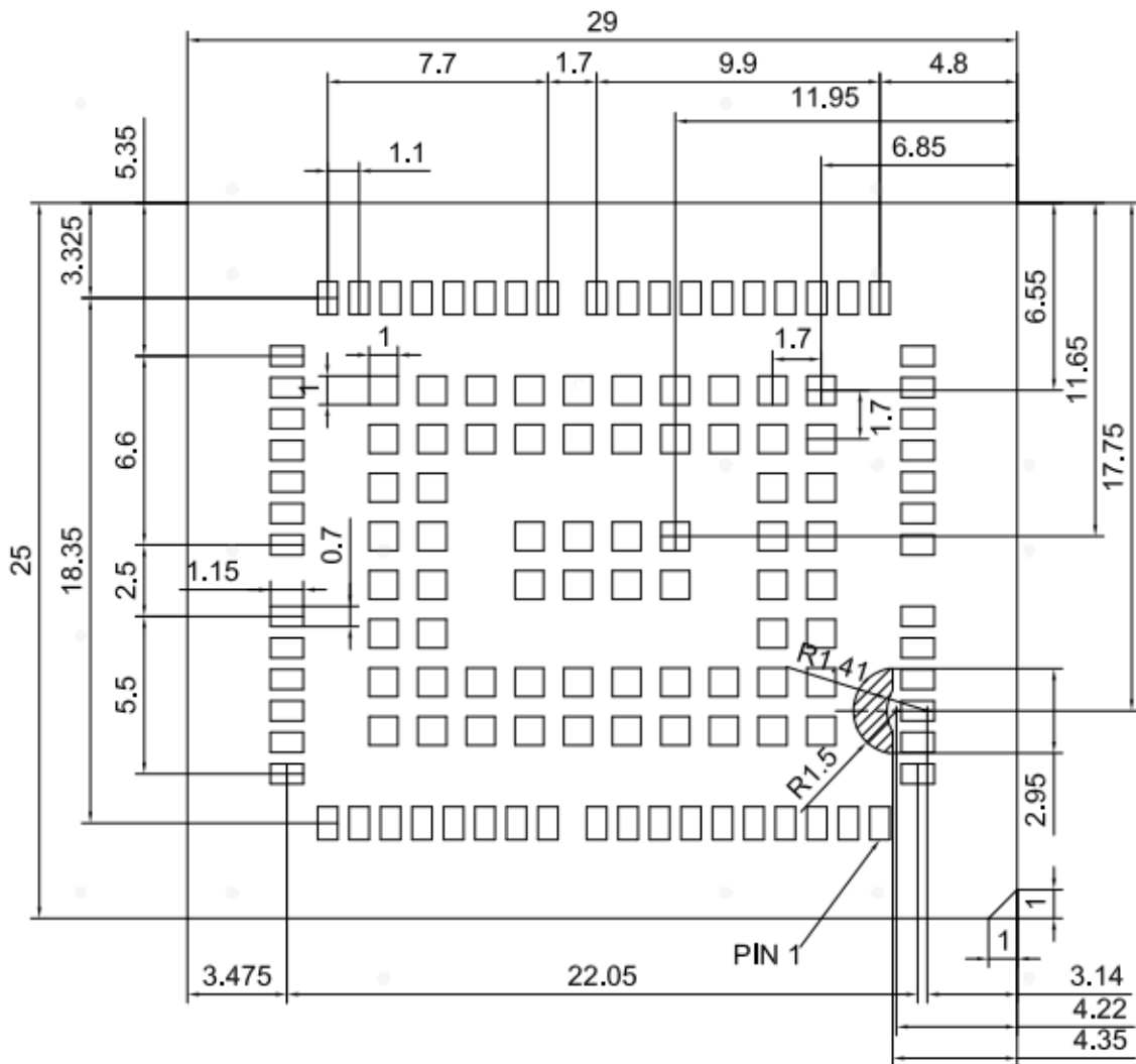
Figure 9-1 N717-EA PCB package (bottom view, unit: mm)
