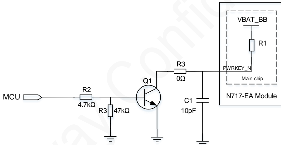
Figure 5-7 Reference design of MCU-control startup
