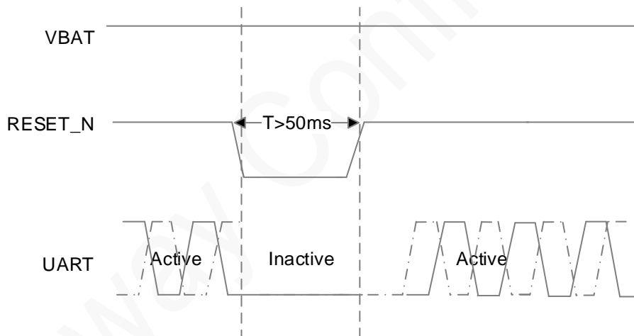
Figure 5-13 Module reset process
