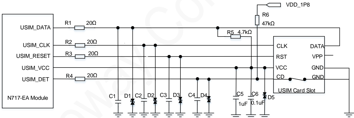
Figure 5-19 Reference design of the USIM interface (normally close connector)
