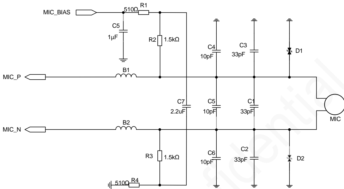
Figure 5-24 Reference design of the differential MIC input
