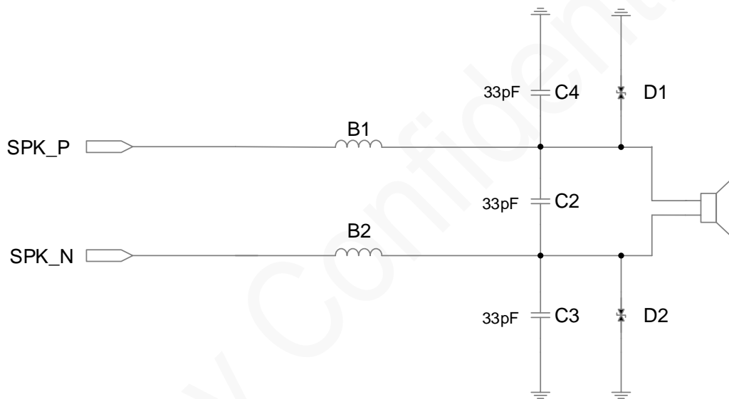
Figure 5-25 Reference design of the differential SPK input
