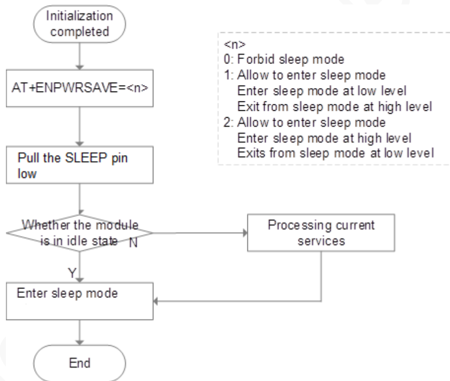
Figure 5-34 Process of entering into sleep mode
