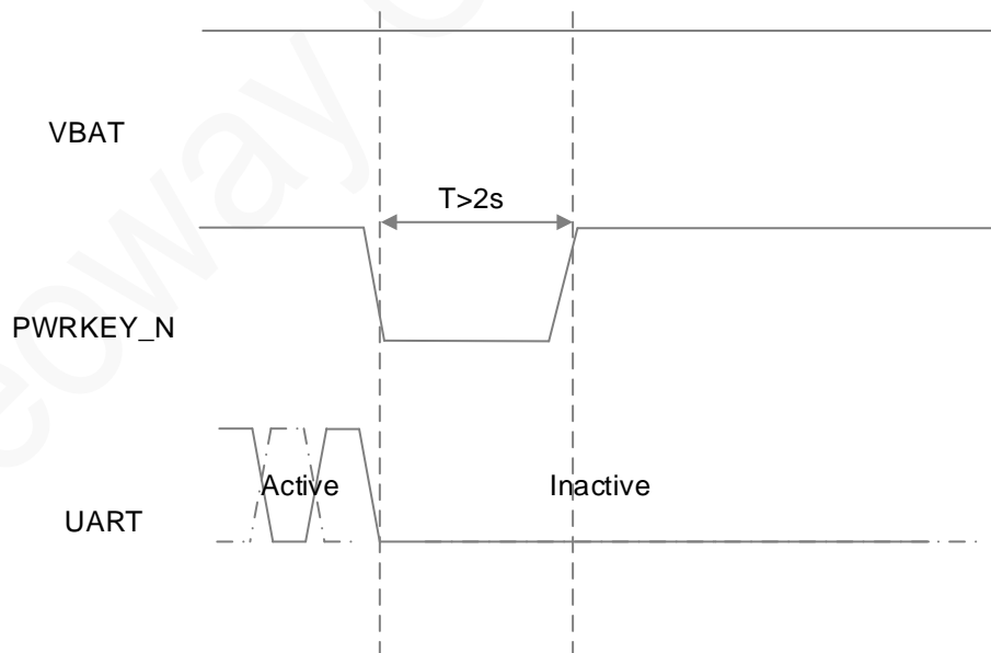
Figure 5-10 N717-EA hardware power-off process
