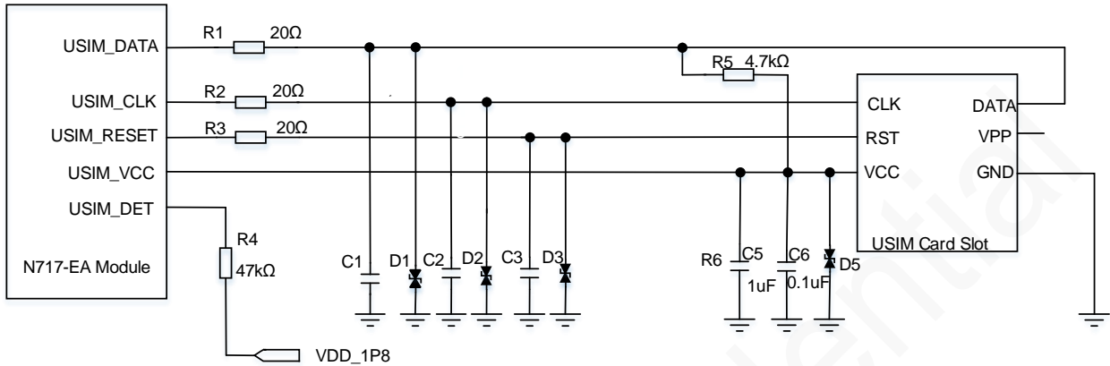
Figure 5-21 Reference design of USIM card interface (without hot-swapping function)
