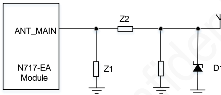
Figure 5-28 \pi -type RF matching schematics
