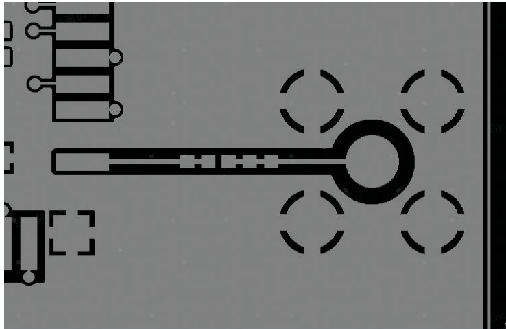
Figure 5-29 Recommended RF PCB design
