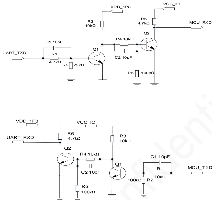
Figure 5-17 Recommended voltage-level translation circuit 2
