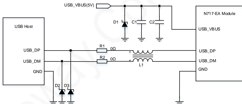
Figure 5-14 Reference design of the USB interface
