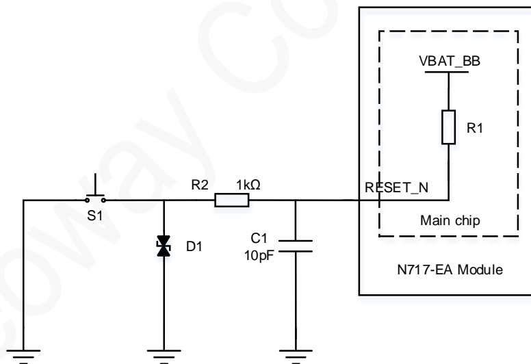
Figure 5-11 Key-control reset
