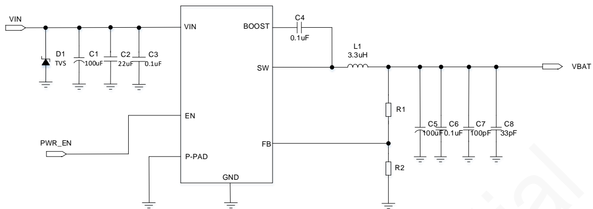
Figure 5-5 Recommended power supply design4
