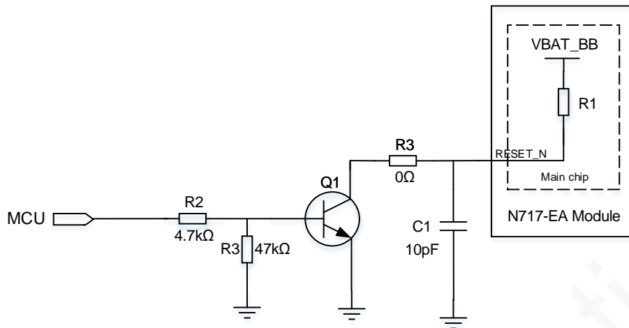
Figure 5-12 MCU-control reset
