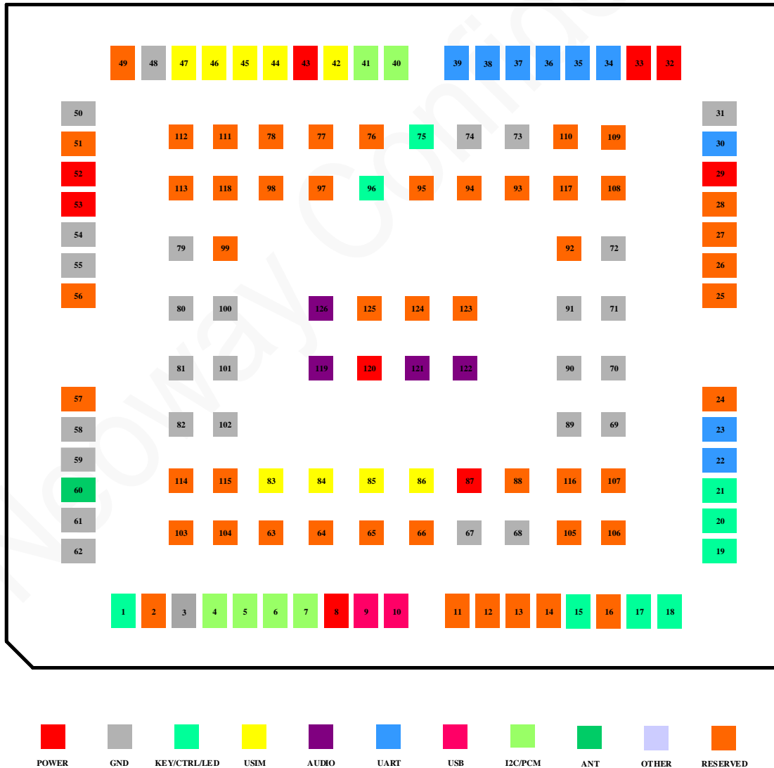
Figure 4-1 N717-EA pad layout (top view)
