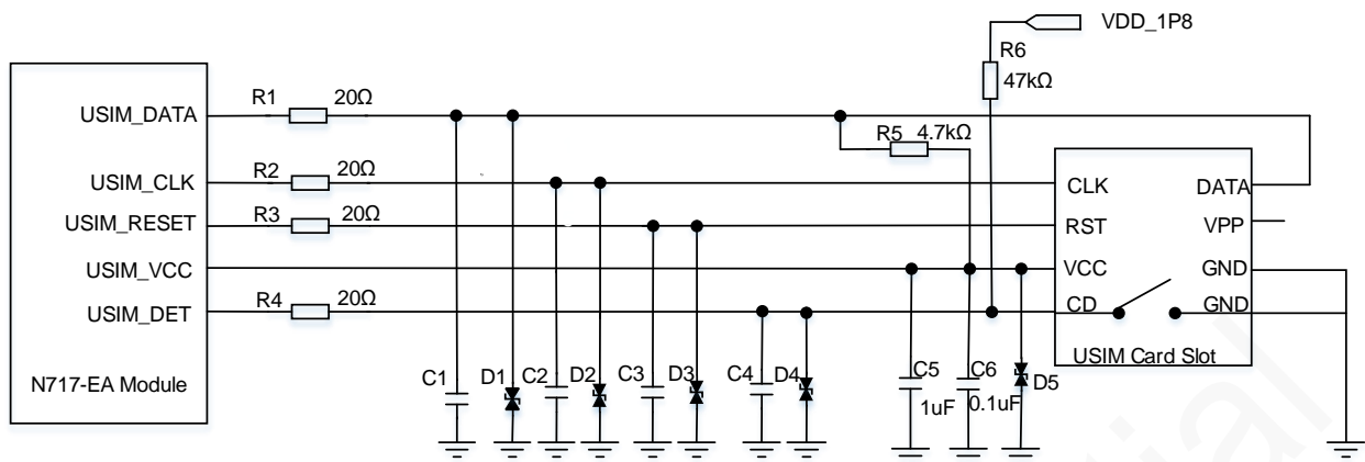
Figure 5-20 Reference design of the USIM interface (normally open connector)
