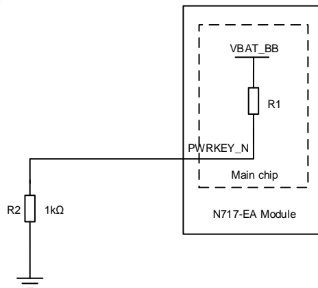
Figure 5-9 Reference design of automatic startup once powered up
