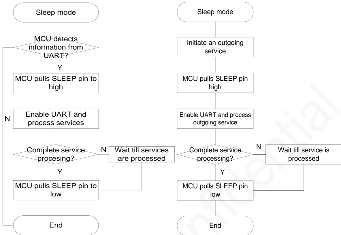
Figure 5-35 Process of processing data services in sleep mode
