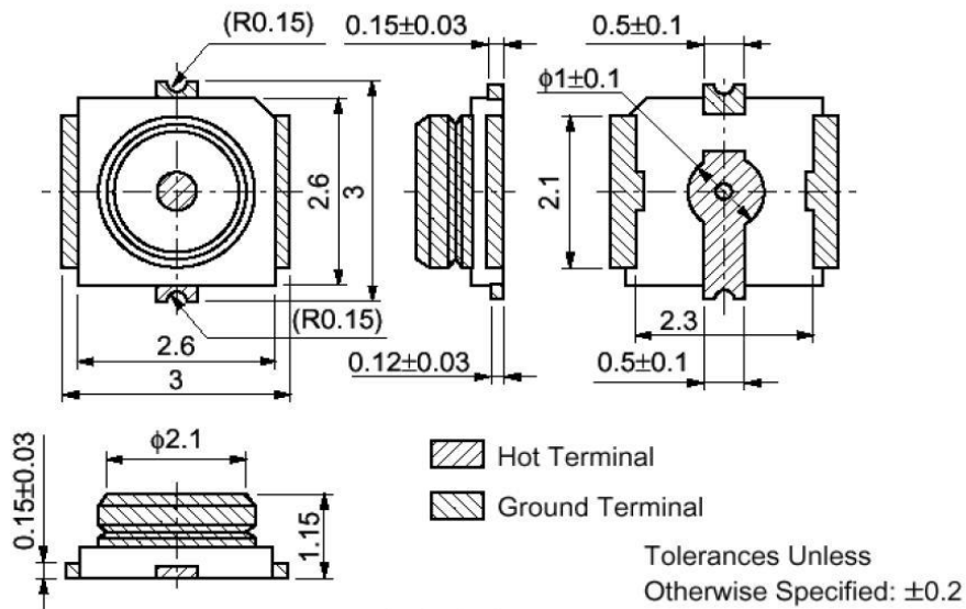
Figure 5-30 Murata RF connector encapsulation specifications
