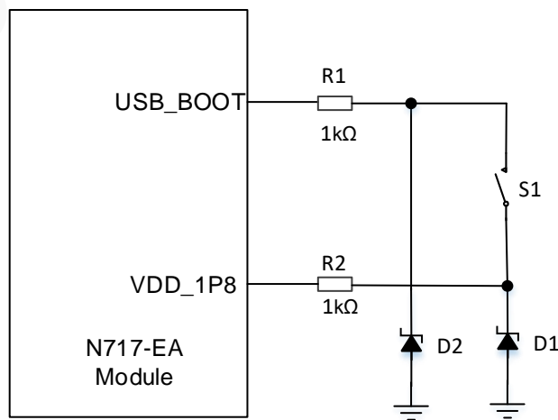
Figure 5-38 Reference design of USB_BOOT pin
