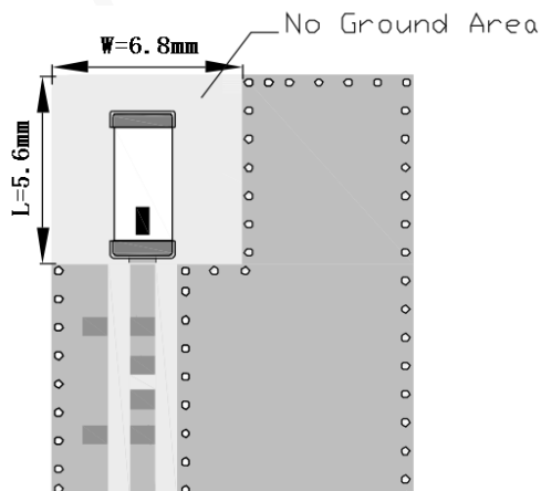
Figure 5-33 Clearance area around the antenna
