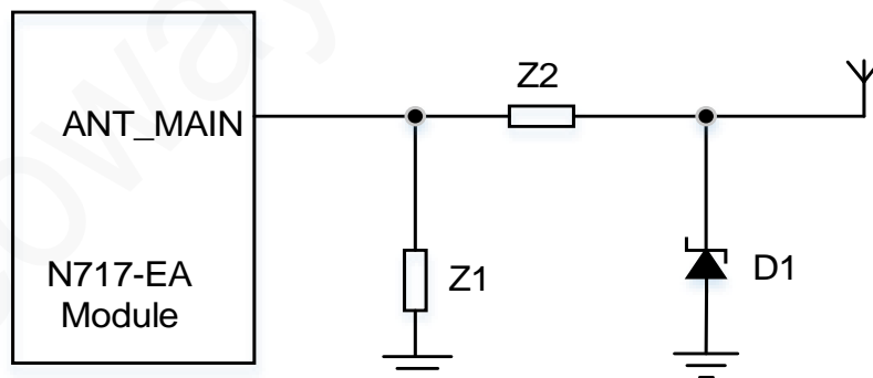
Figure 5-26 L-type RF matching schematics
