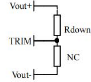
Voltage Down: Add resistor R_{down} between Trim and output positive R_{down} = 43 * (21.5 - \Delta U) / \Delta U - 5.1 \text{ (K}\Omega\text{)}
