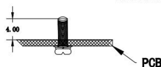
Standard 61*57.9*12.7mm
