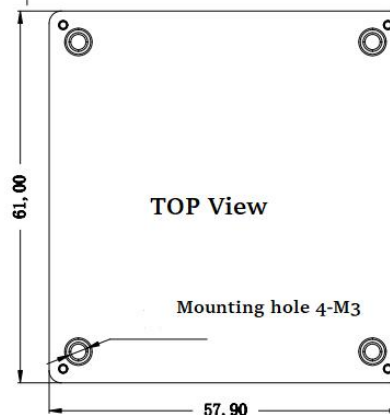
Standard 61*57.9*12.7mm
