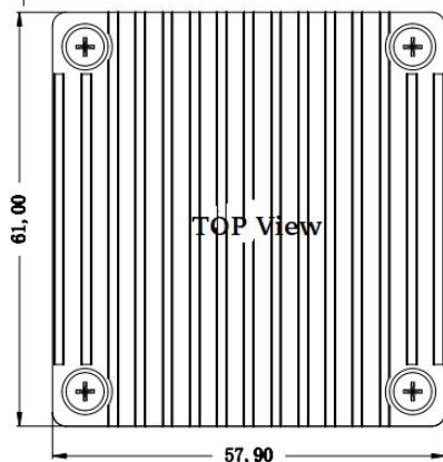
Standard+Heatsink 61*57.9*27.7mm
