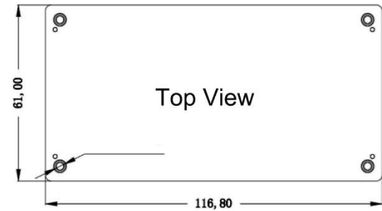
Standard 116.8*61*12.5mm
