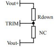
Voltage Down: Add resistor R_{down} between Trim and output positive R_{down} = 20 * (36 - 2.5 - \Delta U) / \Delta U - 5.1 (K \Omega )
